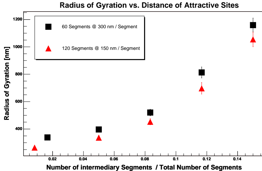
Figure 4. The diameter of the rosettes depends on the number of attractive sites. The different Kuhn lengths are only of minor importance.
