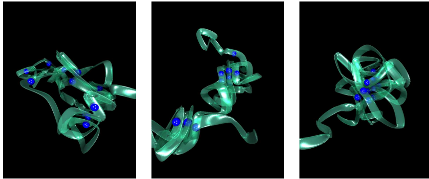
Figure 2. Left: We see the starting configuration of a 60 segment chromatin fibre. The spheres represent the condensing agents. Center: An intermediary configuration. This state of mainly two clusters of approximately equal size turns out to be a metastable state. Right: In the final state all attractive segments are concentrated in the centre. A rosette has formed.
