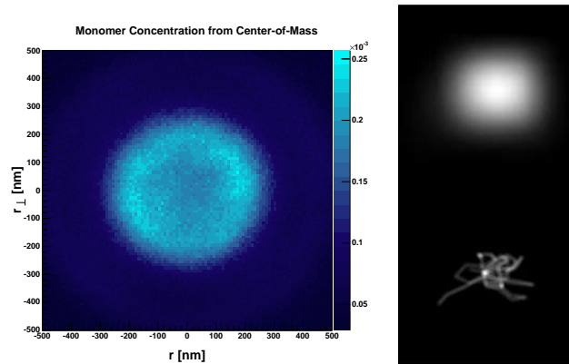
Figure 5. Left: Projection of the average monomer concentration of a rosette with a diameter of about 600 nm. Right: Projections of virtual microscopy image data stacks of one simulated rosette (before convolution with a measured confocal point spread function (bottom) and after convolution (top)).
